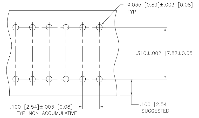
RECOMMENDED MOUNTING HOLE PATTERN SCALE 4/1 FIGURE # 1
